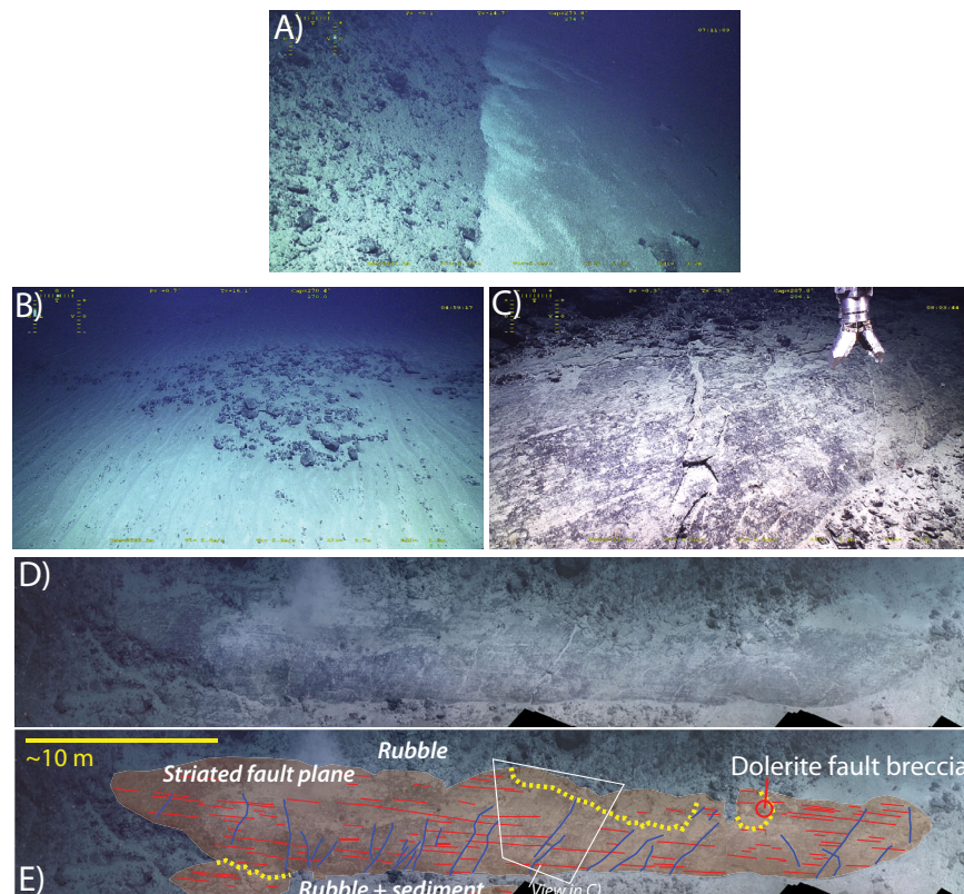
Figure 7. Seafloor images of the 13°20'N corrugated surface. (A) Extension-parallel view (toward the W) of the flank of a corrugation (see location in Figure 6), covered with rubble, and sedimented seafloor at its base (dive 550, field of view ~10 m in foreground). (B) Extension-parallel view (toward the W) of the ridgeward face of a “ripple” ridge crosscutting the corrugation (dive 557, field of view ~15 m in foreground). (C) View of a striated fault plane at the flank of a corrugation (oblique view to striations, see scale and image position in videomosaic in Figure 7E). Striations are subhorizontal and extension-parallel. The fault plane is covered by rubble above, and sediment and rubble at its base. View toward the SSE and see Figure 7E for scale (dive 547). (D) Videomosaic of the ~40 m long striated fault plane in Figure 7C, and (E) the corresponding geologic interpretation (E or ridge axis to the left). Striations are shown in red, fractures at the fault outcrop in blue, and limits of fault surfaces in dashed yellow. The location of a fault breccia sample (diabase) is also indicated.
