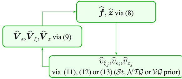
FIGURE 2 – Algorithme itératif Joint MAP
