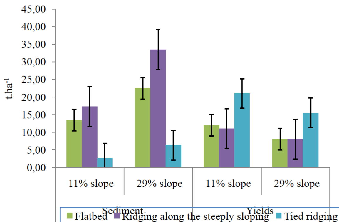
Fig. 1. Chart of average sediment and yields per hectare, per cultivation method and per slope
