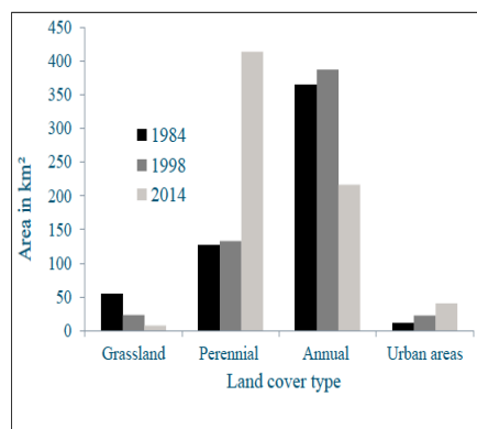
Fig.4. Area of major land cover types in 1984, 1998 and 2014 in the Hawassa area
