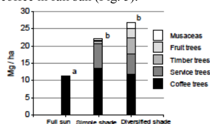
Fig. 5. Above-ground biomass carbon.
