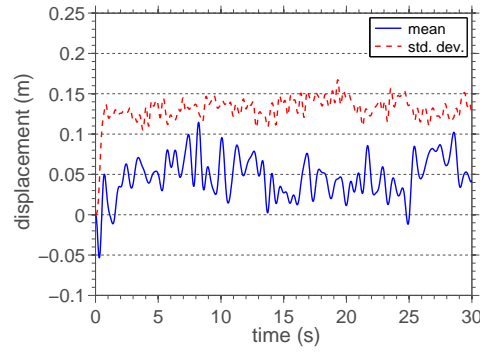
Fig. 7 Sample mean/standard deviation for tower horizontal displacement.
