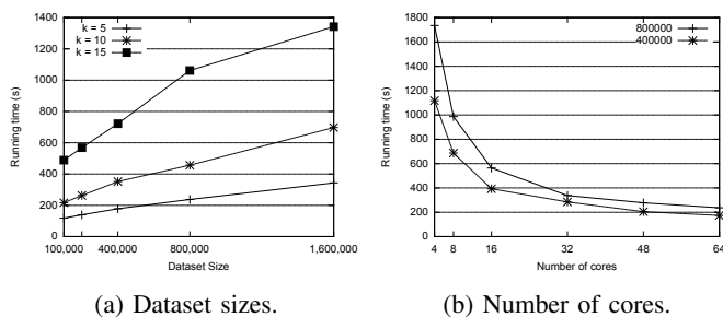
Fig. 3: Scalability. Our approach scales roughly linearly.
