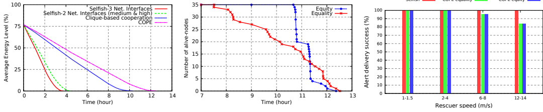
FIGURE 3: Average energy level over time FIGURE 4: Number of alive-nodes over time FIGURE 5: Emergency alert delivery success (all nodes are alive)
