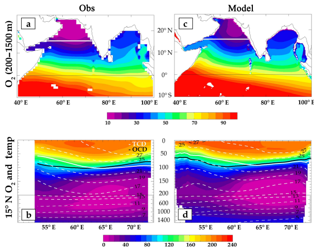
Figure 3. (a) Map of yearly climatological \text{O}_2 concentration ( \mu\text{mol L}^{-1} ) averaged between 200 and 1500 m depths in the northern Indian Ocean from WOA13. (b) The vertical distribution of yearly climatological \text{O}_2 ( \mu\text{mol L}^{-1} ; shaded) and temperature ( ^{\circ}\text{C} ; dashed white contours with 2^{\circ}\text{C} interval) across the east–west section at 15^{\circ}\text{N} (indicated by white line in panels a and c) in the Arabian Sea from WOA13 data. (c, d) Same as (a, b) but for the model. Depths of 23^{\circ}\text{C} isotherm (white line) and of 100 \mu\text{mol L}^{-1} isoline (black line) are marked in panels (b) and (d).
