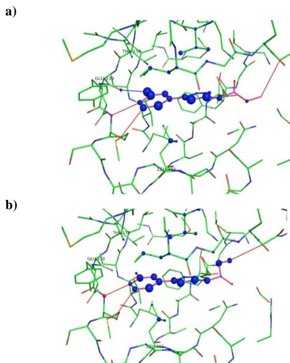
Fig. (3). DSX prediction for compounds 3b (a) and 3m (b). DSX prediction for compounds 3b and 3m blue spheres represents favorable interactions, red spheres represent bad interactions, blue lines represent good distances and red lines bad distances.
