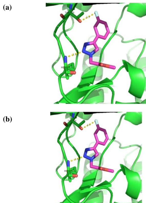
Fig. (4). Binding mode of compound 3k calculated with PLANTS (a) and DSX evaluation (b).
