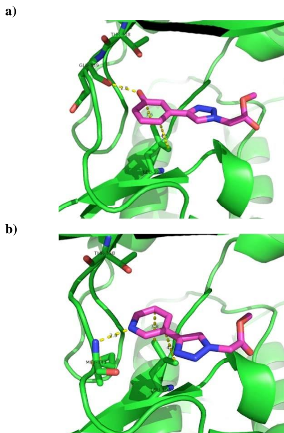
Fig. (2). Binding modes of compounds 3m and 3p calculated with PLANTS.
