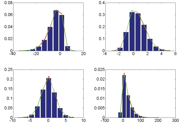
Fig. 4. Marginal posterior distribution from the estimated (green) and true (red) APD parameters in each area of the image in Fig. 3.
