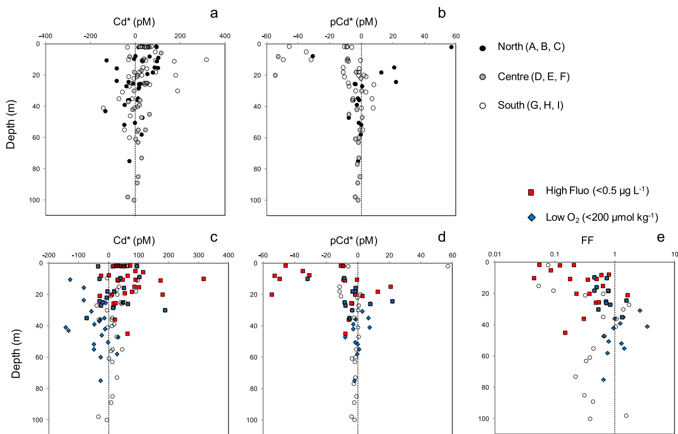
Figure 7. (top) vertical distribution of (a) Cd^* and (b) pCd^* for the northern (black circles), central (grey circles), and southern areas (white circles). Cd^* is defined as Cd^* = Cd_{measured} - 0.25 \times P_{measured} , and pCd^* as pCd^* = pCd_{measured} - 0.25 \times pP_{measured} , 0.25 being the Cd:P ratio of NACW [Yeats et al. , 1995]. (bottom) Vertical distribution of (c) Cd^* , (d) pCd^* , and (e) fractionation factor (FF) with FF = (pCd:pP)/(Cd:PO_4) [Elderfield and Rickaby, 2000] for fluorescence concentrations greater than 0.5 \text{ mg m}^{-3} (red squares) and for low dissolved oxygen concentrations ( <200 \text{ } \mu\text{mol kg}^{-1} ). White circles correspond to samples that did not fall into the conditions above mentioned.
