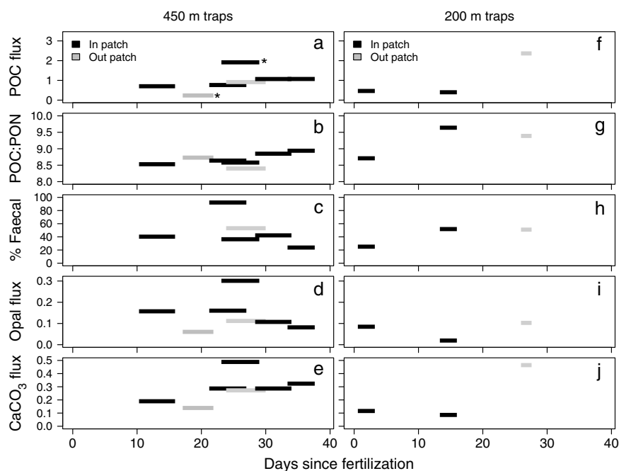
Figure 6. Fluxes intercepted by PELAGRA sediment traps. Each horizontal line represents one trap, with the line's length indicating the collection period. (a–e) Results from 450 m traps. (f–j) Results from 200 m traps. Note that the very low POC flux measured in trap D4#470 is probably erroneous, while the samples in trap D6#440 were compromised because the trap could not be recovered until 48 h after surfacing (see section 3). These data are marked with asterisks.
