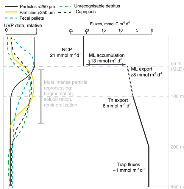
Figure 8. Overview of carbon fluxes and particle profiles during LOHAFEX. The right side summarizes the carbon fluxes: NCP averaged 21 \text{ mmol m}^{-2} \text{ d}^{-1} in the mixed layer, of which \leq 13 \text{ mmol m}^{-2} \text{ d}^{-1} accumulated in the mixed layer, leaving at least 8 \text{ mmol m}^{-2} \text{ d}^{-1} for export below the mixed layer. The dotted line indicates that mixed layer export is not very well constrained, and thus, the degree of flux attenuation between the mixed layer and 100 m is uncertain. ^{234}\text{Th} -derived export exceed the flux caught in sediment traps, indicating further attenuation from 100 to 200 m. The left side of the figure summarizes the UVP data, with abundance of different particle types indicated on a relative axis. The UVP data collectively indicate that particle transformation was most intense between the base of the mixed layer and 150 m, most likely owing to zooplankton activity; flux attenuation was most likely intense throughout this range.
