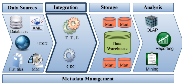
Fig. 1 Data warehousing/business intelligence process
