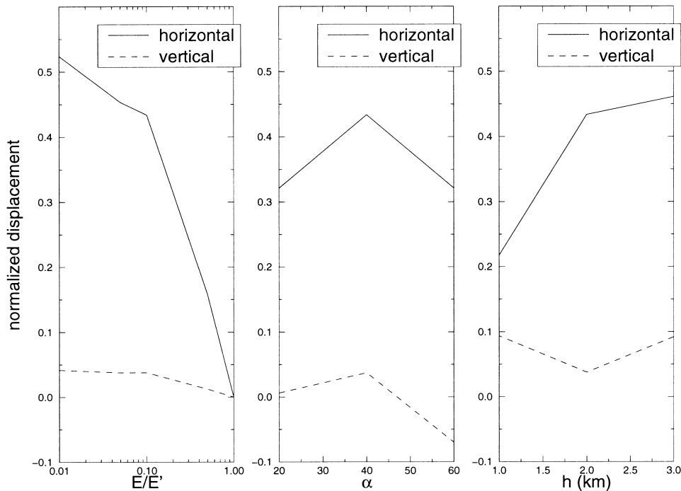
Figure 8. Normalized displacement variations with E , \alpha and h . The low-rigidity layer has a larger influence on the horizontal displacements than on the vertical displacements.
