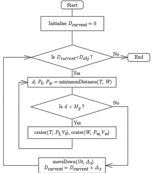
Figure 4. Global overview of the simulation process.
