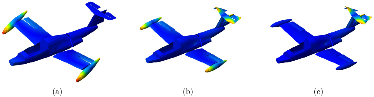
Figure 6: FEP of the first symmetric wing torsional NNM of the Paris aircraft. NNM motions (a) on the backbone (in the vicinity of the branch); (b) in the middle of the branch of 3:1 internal resonance between the first wing torsional mode and a higher tail mode; and (c) at the extremity of the branch. Figure reproduced from [69].
