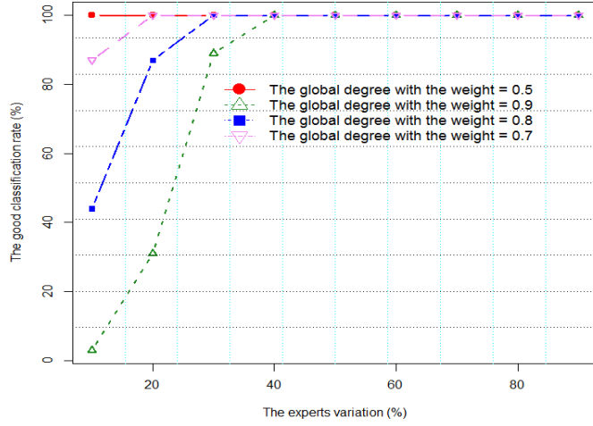
Fig. 1. Variation of the good classification rate according to the percentages of experts
