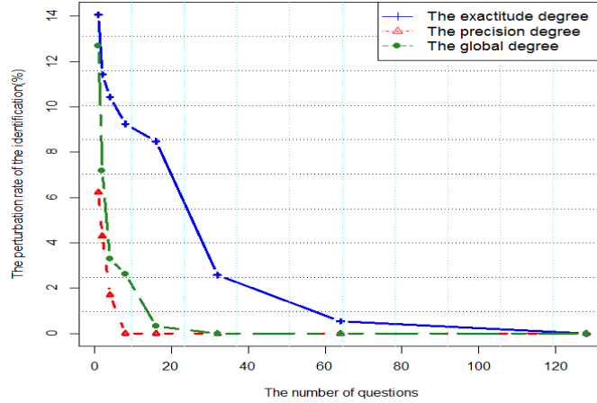
Fig. 2. The variation of the perturbation rate according to the different degrees
