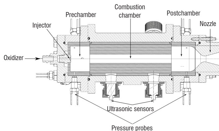
Figure 3 - HYCOM lab-scale engine (left) and schematic view of this facility (right)
