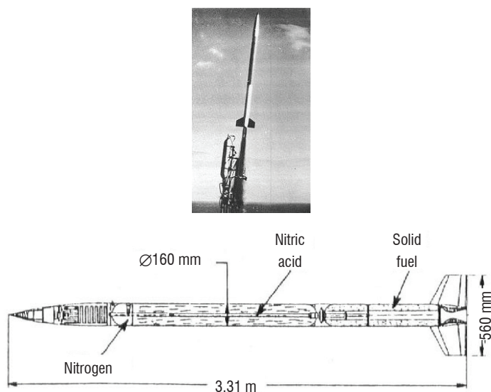
Figure 10 - LEX02 sounding rocket section (bottom) and flight test (top)
