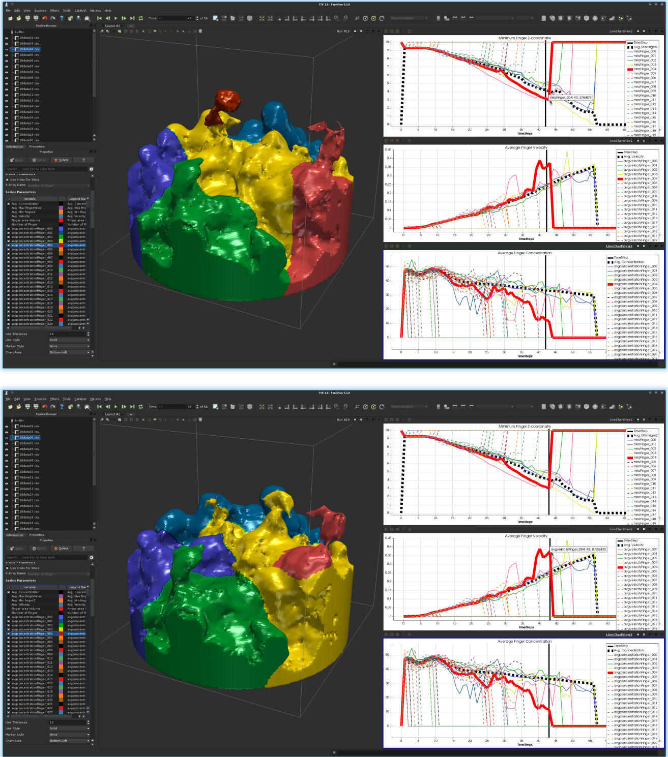
Figure 16: Finger detachment (dark red finger) at time-step 43 of Run #4 (top: before, bottom: after). The 3D linked views show a clear prominence of the dark red finger, despite a the very thin portion that connects it to the rest of the dissolving salt \mathcal{S} . This portion becomes so thin at time-step 43 that this finger gets disconnected from \mathcal{S} and is therefore no longer considered as a finger by our analysis pipeline. We call such a phenomenon detachment , since a rapid finger grows so fast that it detaches from the rest of dissolving salt \mathcal{S} and rapidly vanishes in the ambient water. Time varying statistics are provided on the right side: minimum of Z-coordinate for each finger and average velocity for each finger and average salt concentration for each finger. These curves are shown with dash lines for fingers which are no longer active at the current time step. The bold black dash lines indicate global statistics for the region of dissolving salt \mathcal{S} . The bold, dark red curves indicate time-varying statistics for the dark red finger. In particular, these curve show that, before detachment, this finger was both the deepest down the domain (top curves) and the fastest (center curves). Moreover, the bottom curves show that this finger had a dramatic drop down of salt concentration (bottom curves) exactly when it started to accumulate speed (time-step 38), to eventually fully dissolve in the ambient water.
