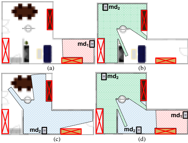
Fig. 7. ILP solution for Z_{C_1} : (a) zone covered by md_1 placed at grid point 465; (b) zone covered by md_2 placed at grid point 5; (c) zone covered by md_2 placed at grid point 636; (d) complete coverage of Z_{C_1} .
