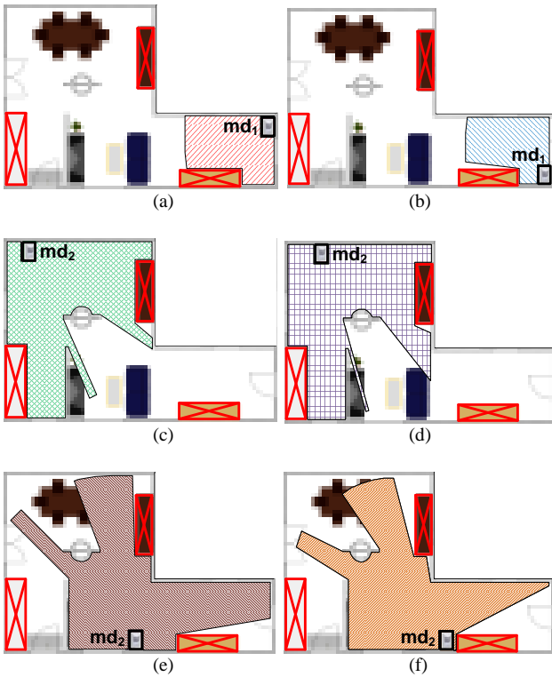
Fig. 11. ILP solution for Z_{c1} : (a) zone covered by md_1 placed at grid point 465; (b) zone covered by md_1 placed at grid point 620; (c) zone covered by md_2 placed at grid point 4; (d) zone covered by md_2 placed at grid point 5; (e) zone covered by md_2 placed at grid point 636; (f) zone covered by md_2 placed at grid point 637.
