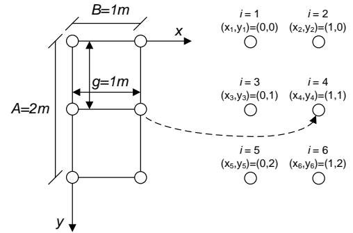
Fig. 5. The 2D grid description of a simple zone (2m \times 1m) .
