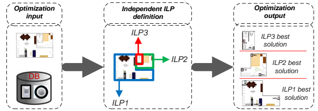
Fig. 1. Sensor placement optimization approach
