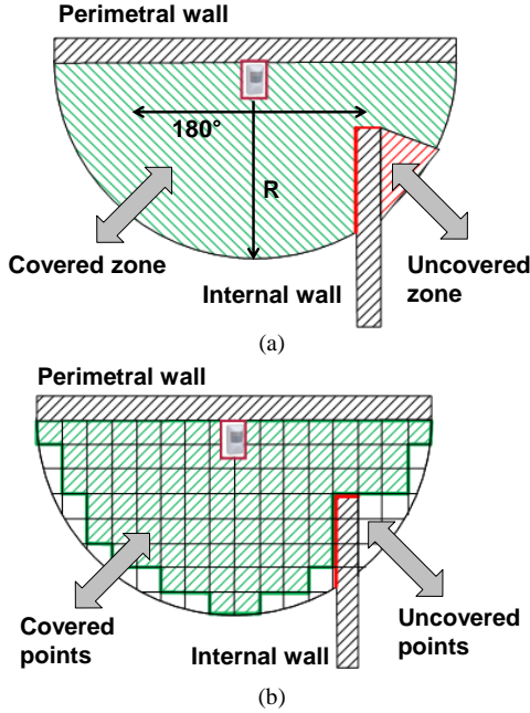
Fig. 3. Motion detectors coverage including obstacles: (a) coverage zone; (b) coverage points on the grid.
