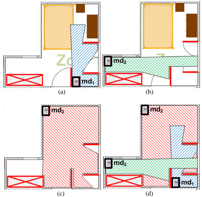
Fig. 10. ILP solution for Z_{C_2} : (a) zone covered by md_1 sensor placed at grid point 436; (b) zone covered by md_2 sensor placed at grid point 337; (c) zone covered by md_2 sensor placed at grid point 10; (d) complete coverage of Z_{C_2} .
