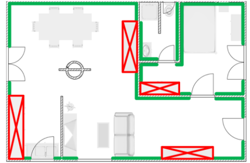
Fig. 6. The perimeter walls available for motion detectors placement.
