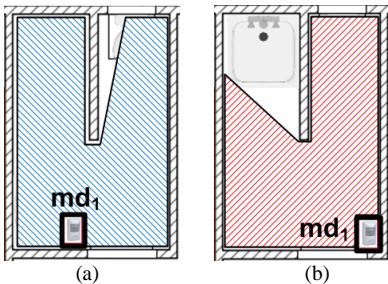
Fig. 9. The ILP solution for Z_{C_3} : (a) zone covered by md_1 placed at grid point 390; (b) zone covered by md_1 placed at grid point 398.
