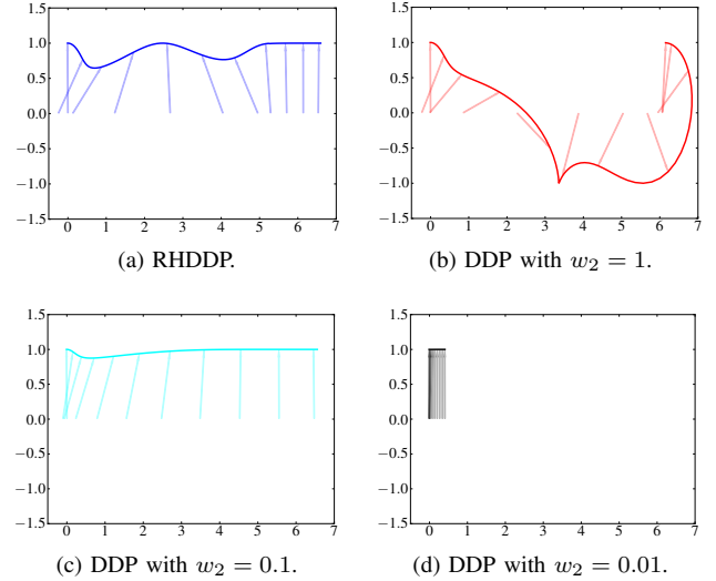
Fig. 8. Test 3: trajectory of the cart-pole system obtained with the different algorithms. The cart start at position 0 and should move to position 6.
