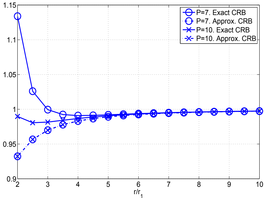
Fig.5 Approximate and exact ratios \text{CRB}(\phi)/\text{CRB}_{\text{FF}}(\phi) for the UCA.
