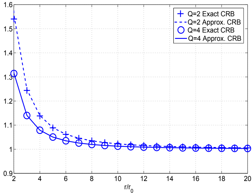
Fig.7 Approximate and exact ratios \text{CRB}(\theta)/\text{CRB}_{\text{FF}}(\theta) for uniform square-based arrays.
