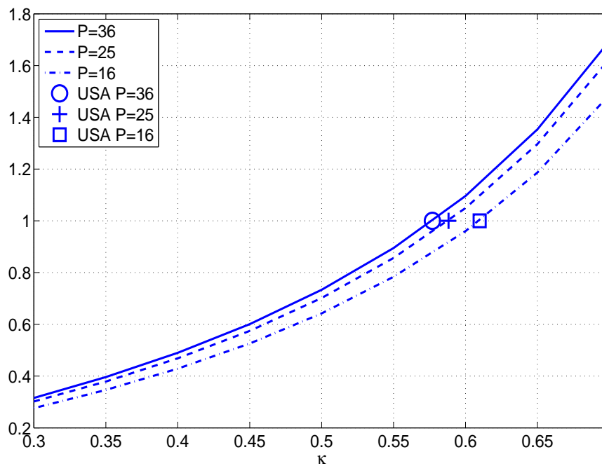
Fig.12 \mathcal{R}_P(\kappa) as a function of \kappa for different square-based centro-symmetric arrays for \theta = 60^\circ and \phi = 30^\circ .
