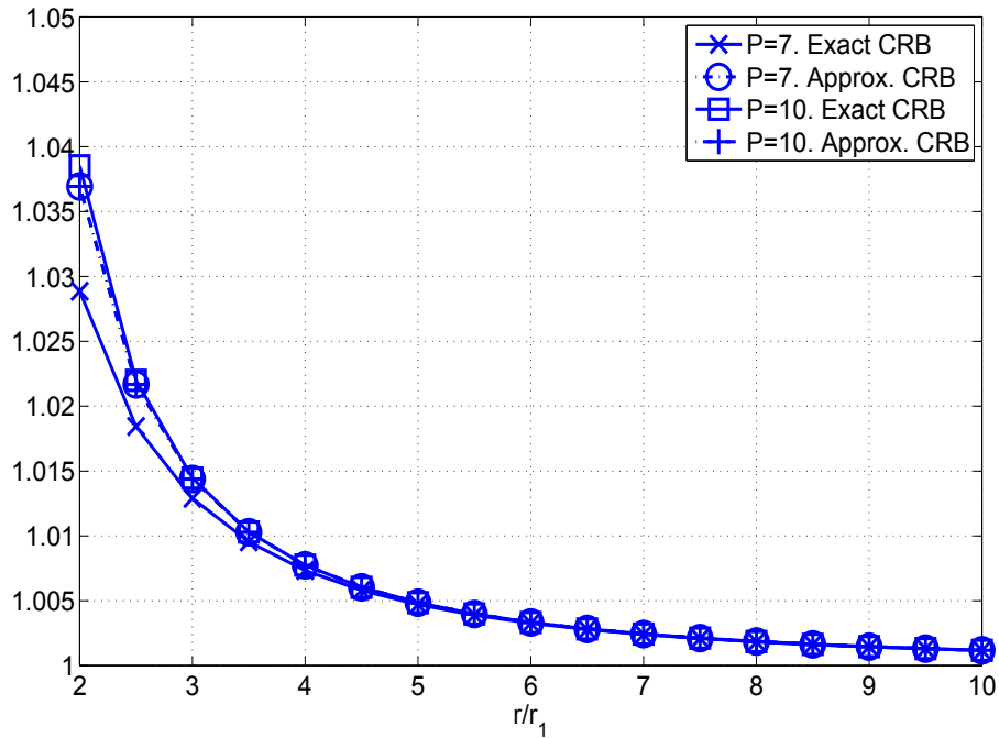
Fig.4 Approximate and exact ratios \text{CRB}(\theta)/\text{CRB}_{\text{FF}}(\theta) for the UCA.
