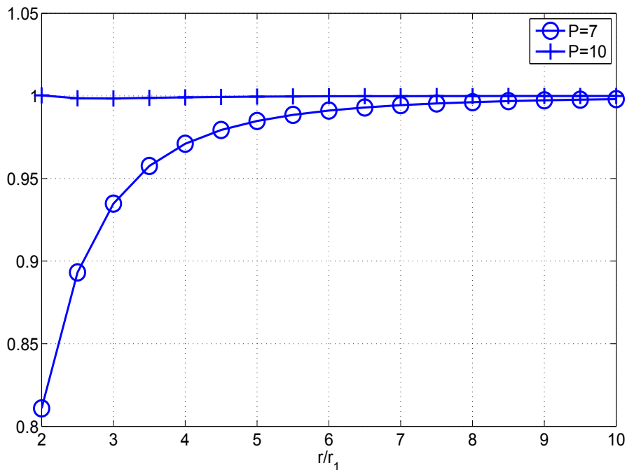
Fig.6 Ratio of the approximate \text{CRB}(r) to the exact one for the UCA.
