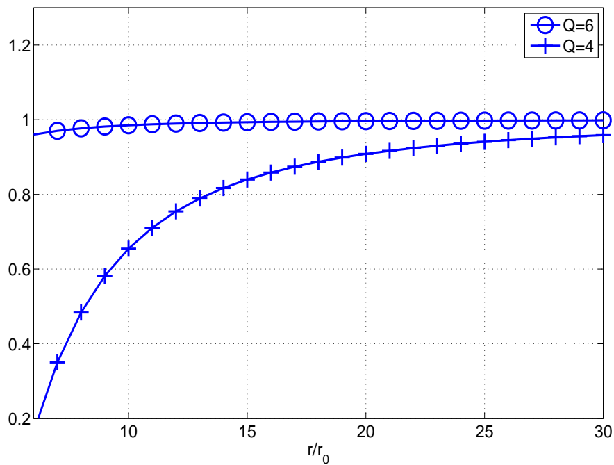
Fig.9 Ratio of the approximate \text{CRB}(r) to the exact one for uniform square-based arrays.
