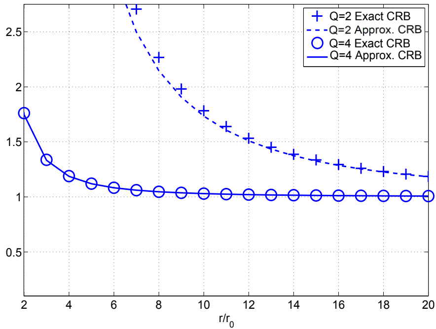
Fig.8 Approximate and exact ratios \text{CRB}(\phi)/\text{CRB}_{\text{FF}}(\phi) for uniform square-based arrays.
