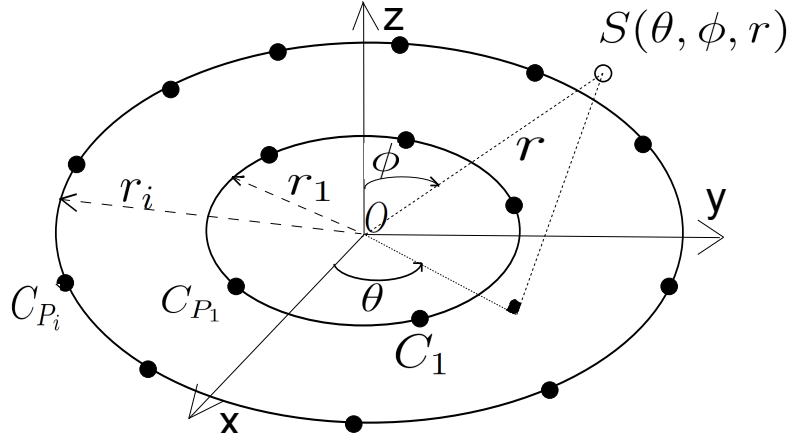
Fig.1 Concentric uniform circular-based array and source parameters.
