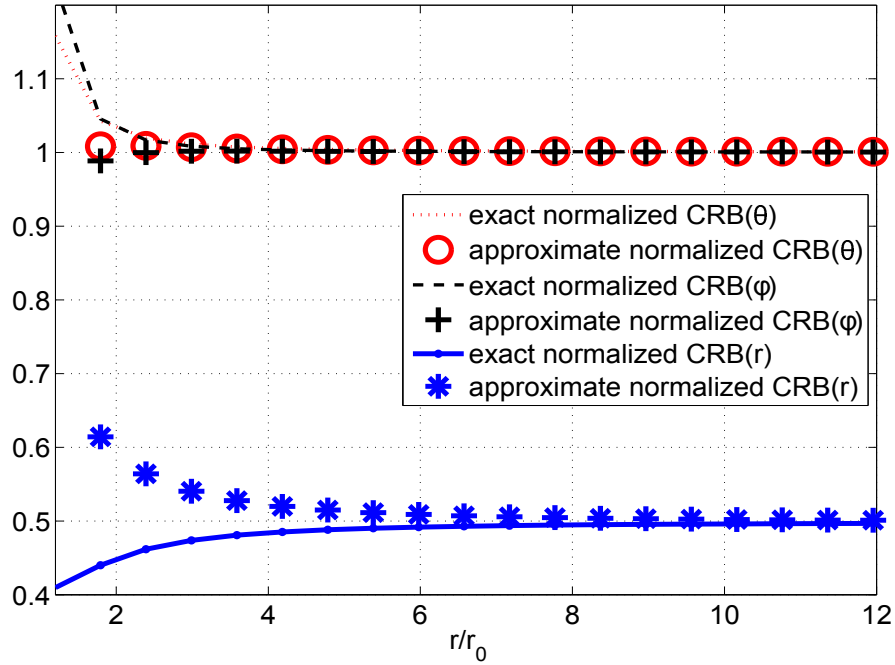
Fig.14 Azimuth, elevation and range CRBs of a square-based centro-symmetric arrays with \kappa_{nu} = 0.4000 normalized to that of the equivalent USA ( \kappa_u = 0.5776 ). Both arrays are made of P = Q^2 = 36 sensors
