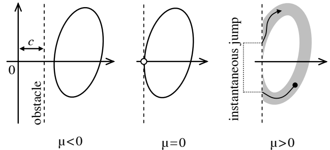
Figure 14: A stable periodic solution that exists for \mu < 0 collides with the obstacle when \mu = 0 . A grazing bifurcation occurs at this point, leading to the appearance of a trapping region (drawn in gray) for small \mu > 0 . This trapping region may contain stable periodic orbits.
