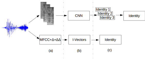
Figure 1: A simplified overview of the system, which highlights how the convolutional neural network was used in this study in contrast to a more traditional approach.
