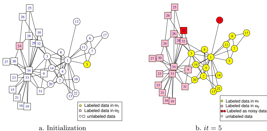
Figure 2. The results on Karate Club network. The nodes marked with color red are the outliers detected by SELP.
