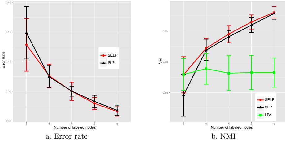
Figure 3. The results on American football network. The two figures show the average error rates and NMI values (plus and minus one standard deviation) for 50 repeated experiments, as a function of the number of labeled samples.
