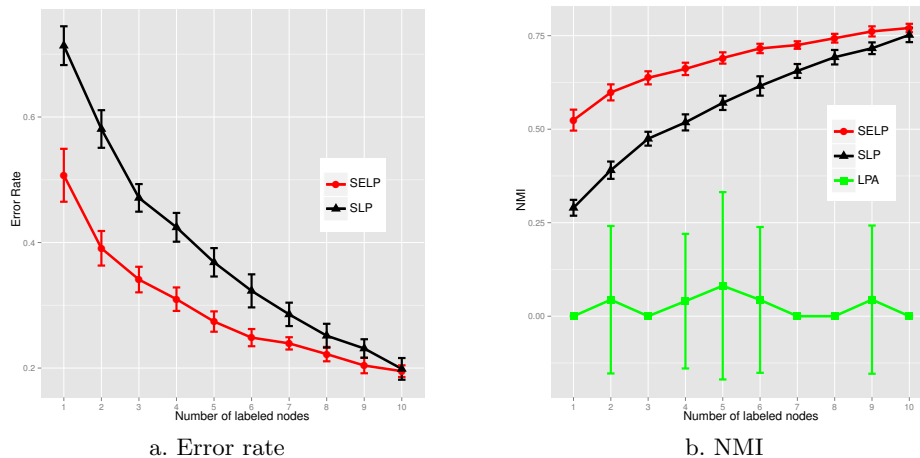
Figure 5. The results on LFR network. The parameter of \mu is set to be 0.6.
