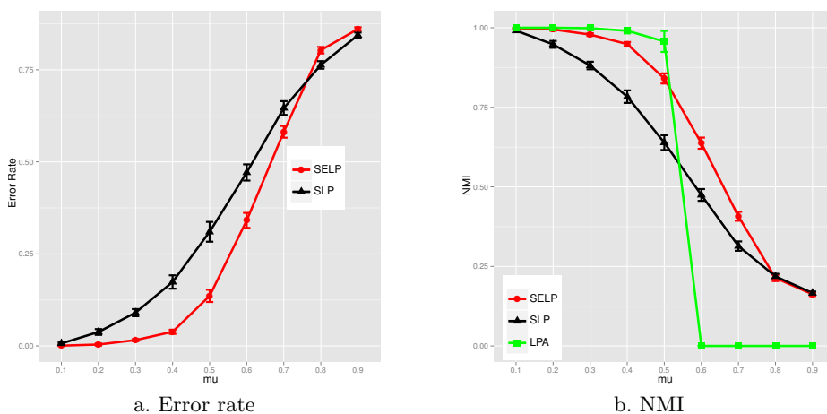
Figure 4. The results on LFR network. The number of labeled nodes in each community is 3.
