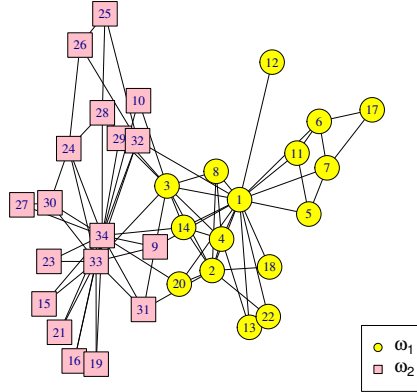
Figure 1. Karate Club network.
