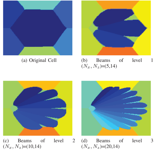
Fig. 2: Multilevel beam coverage maps.
