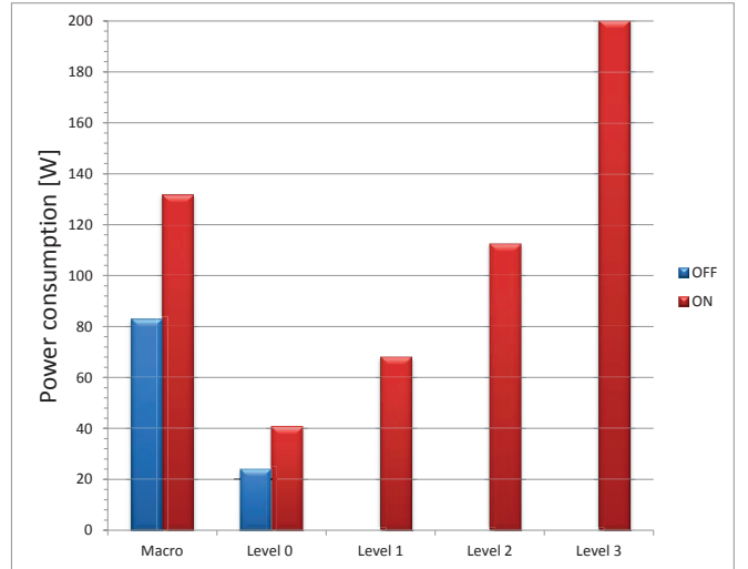
Fig. 3: Power consumption values (Watt). The terms ON and OFF stand respectively for the cases with and without traffic in the cell.
