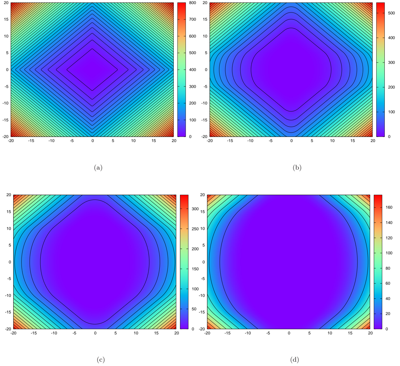
FIGURE 3. Evaluation of the solution \phi((x_1, x_2, 0, 0, 0, 0, 0)^\dagger, t) of the HJ-PDE with initial data J = \frac{1}{2} \|\cdot\|_1^2 and Hamiltonian H = \|\cdot\|_D , for (x_1, x_2) \in [-20, 20]^2 for different times t . Plots for t = 0, 5, 10, 15 are respectively depicted in (a), (b), (c) and (d). The level lines multiple of 20 are superimposed on the plots.
