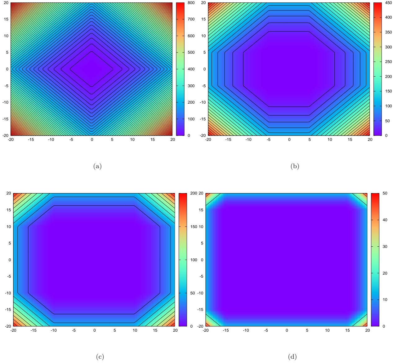
FIGURE 2. Evaluation of the solution \phi((x_1, x_2, 0, 0, 0, 0, 0)^\dagger, t) of the HJ-PDE with initial data J = \frac{1}{2} \|\cdot\|_1^2 and Hamiltonian H = \|\cdot\|_1 for (x_1, x_2) \in [-20, 20]^2 for different times t . Plots for t = 0, 5, 10, 15 are respectively depicted in (a), (b), (c) and (d). The level lines multiple of 20 are superimposed on the plots.
