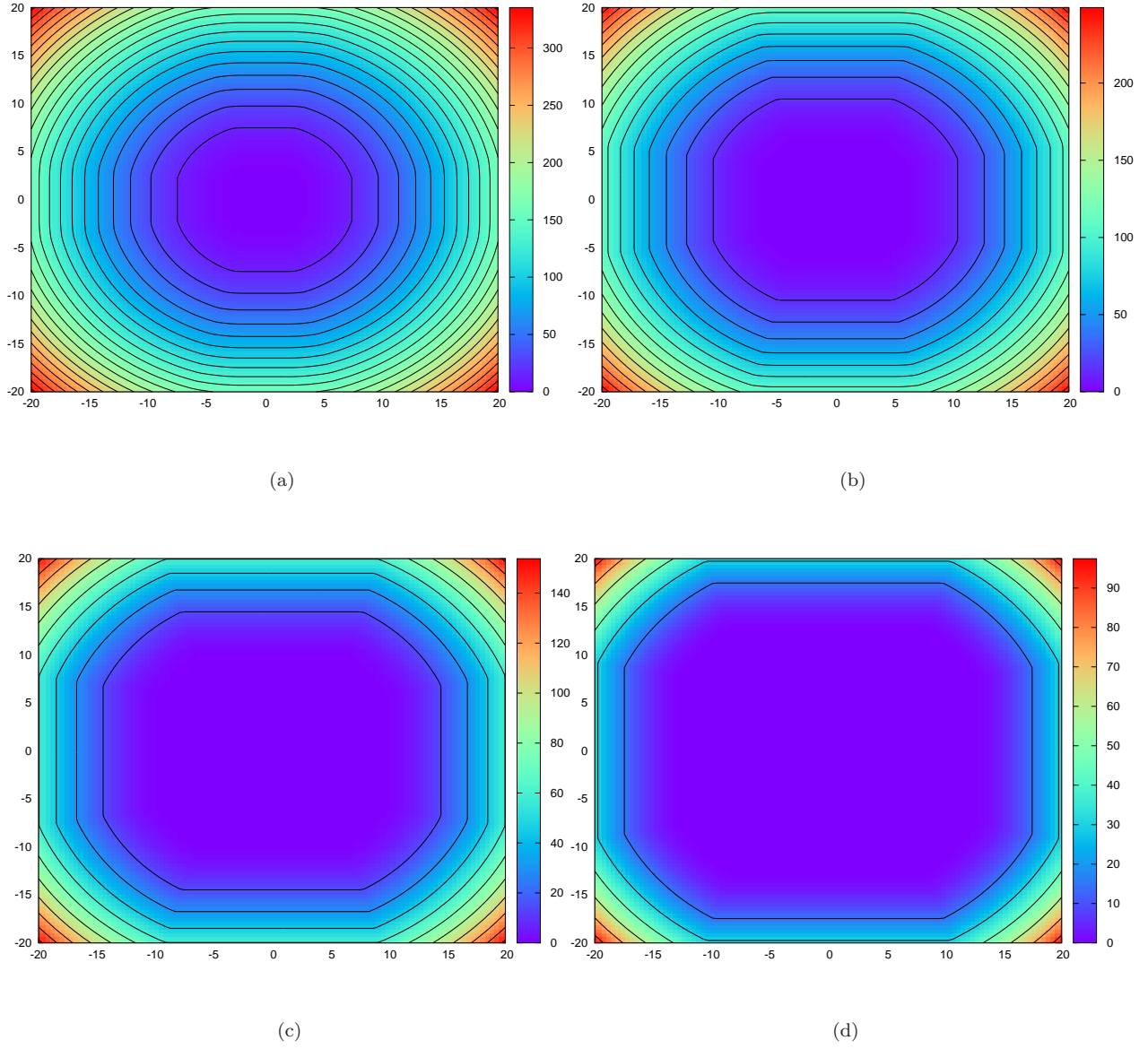
FIGURE 5. Evaluation of the solution \phi((x_1, x_2, 0, 0, 0, 0, 0)^\dagger, t) of the HJ-PDE with initial data J = \frac{1}{2}\|\cdot\|_1^2 and Hamiltonian H = \min\left(\|\cdot\|_1, \sqrt{\langle \cdot, \frac{4}{3}D \cdot \rangle}\right) , for (x_1, x_2) \in [-20, 20]^2 for different times t . Plots for t = 2, 5, 9, 12 are respectively depicted in (a), (b), (c) and (d). The level lines multiple of 15 are superimposed on the plots.
