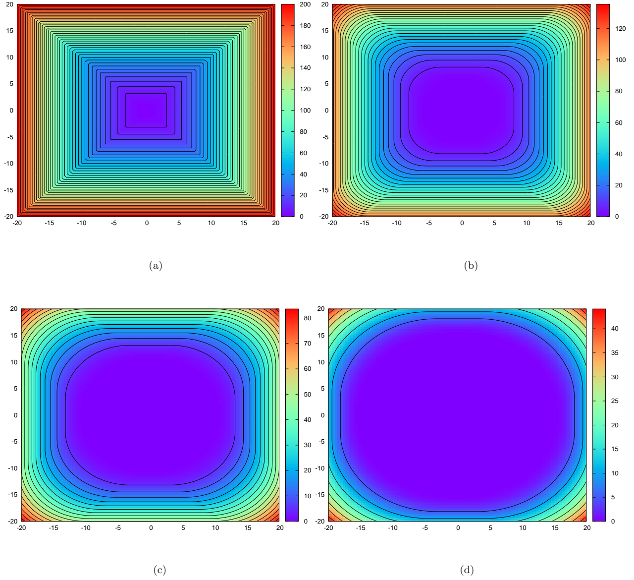
FIGURE 1. Evaluation of the solution \phi((x_1, x_2, 0, 0, 0, 0, 0)^\dagger, t) of the HJ-PDE with initial data J = \frac{1}{2} \|\cdot\|_\infty^2 and Hamiltonian H = \|\cdot\|_2 for (x_1, x_2) \in [-20, 20]^2 for different times t . Plots for t = 0, 5, 10, 15 and respectively depicted in (a), (b), (c) and (d). The level lines multiple of 5 are superimposed on the plots.
