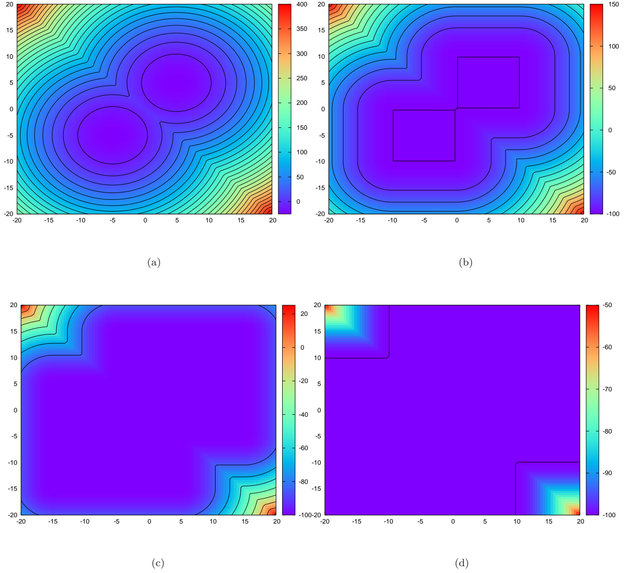
FIGURE 4. Evaluation of the solution \phi((x_1, x_2, 0, 0, 0, 0, 0)^\dagger, t) of the HJ-PDE with initial data J = \min \left( \frac{1}{2} \|\cdot\|_2^2 - \langle b, \cdot \rangle, \frac{1}{2} \|\cdot\|_2^2 + \langle b, \cdot \rangle \right) with b = (1, 1, 1, 1, 1, 1, 1)^\dagger and Hamiltonian H = \|\cdot\|_1 , for (x_1, x_2) \in [-20, 20]^2 for different times t . Plots for t = 0, 5, 10, 15 are respectively depicted in (a), (b), (c) and (d). The level lines multiple of 15 are superimposed on the plots.
