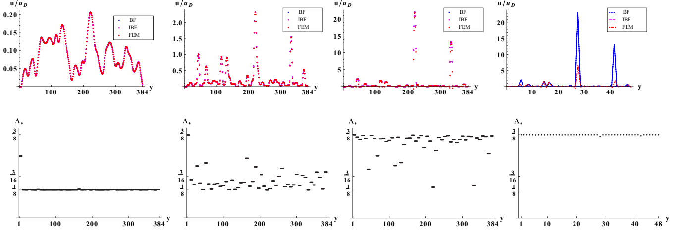
FIG. 30. (Color online) Top row: Velocity distribution in ML1 with BF (blue), IBF (magenta), and FEM (red), with \sigma = \text{Da}^{-1/2} = \{15.2, 152, 1520, 15200\} from left to right. In the fourth diagram, BF and IBF almost coincide, and FEM is shown in a dot-dashed line. Grid refining h = 8 except for the last diagram, where h = 1 . Bottom row: Corresponding effective distribution \Lambda_* in IBF given by Eq. (55). The BF/IBF are applied with \Lambda = \frac{1}{8} in the three first cases and \Lambda = \frac{1}{64} in the last diagram where \Lambda_* \rightarrow \frac{3}{8} when \sigma \rightarrow \infty .
