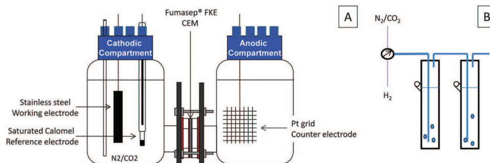
Fig. 1 Experimental set-up of (A) the microbial electrochemical reactor – MER and (B) the gas-liquid contactor – GLC.
