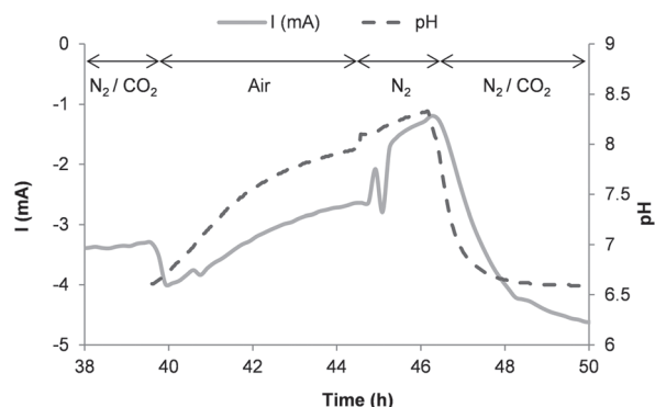
Fig. 5 Evolution of the pH due to different gas injection with or without carbon dioxide gas and the concomitant variation in intensity at a stainless steel cathode polarized at -0.66 V vs. SHE.
