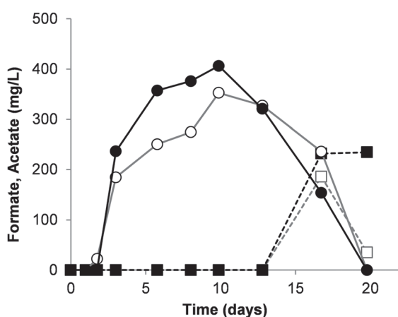
Fig. 8 Formate (round) and acetate (square) production in 2 gas-liquid contactors inoculated with the salt marsh sediment and fed with 10 \text{ mL min}^{-1} N_2-CO_2 gas mixed with 6 \text{ mL min}^{-1} H_2 .
