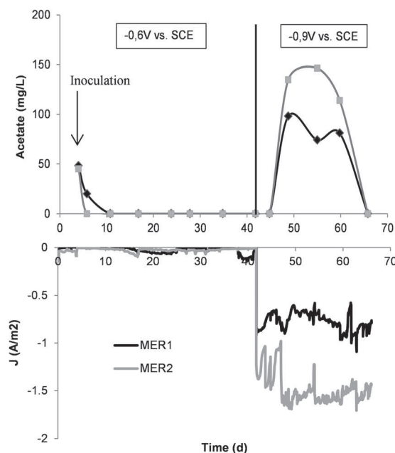
Fig. 2 Production of acetate and associated chronoamperometry in MERs initially polarized at -0.36 \text{ V vs. SHE} for 40 days and then switched to -0.66 \text{ V vs. SHE} . On the 4th day, the MERs were inoculated with the acclimated sludge.
