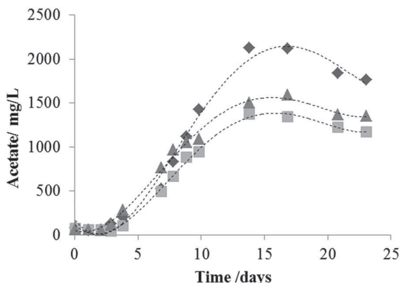
Fig. 7 Acetate production in 3 improved gas-liquid contactors (triplicate) inoculated with the acclimated activated sludge and fed with H_2 at 0.5 \text{ mL min}^{-1} and N_2-CO_2 at 10 \text{ mL min}^{-1} .
