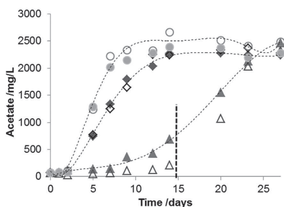
Fig. 6 Acetate production in 6 gas-liquid contactors inoculated with the acclimated activated sludge and fed with N 2 /CO 2 gas mixed with different H 2 flow rates. H 2 was injected at 6 mL min -1 in GLCs 5-6 (round), 2 mL min -1 in GLCs 3-4 (square) and with alternating supply in GLCs 1-2 (triangle) during first 15 days. The dotted line represents the switch in the feeding mode for GLCs 1-2: from the alternating mode to continuous feeding at 2 mL min -1 . Each reactor was continuously fed with N 2 -CO 2 at 10 mL min -1 .
