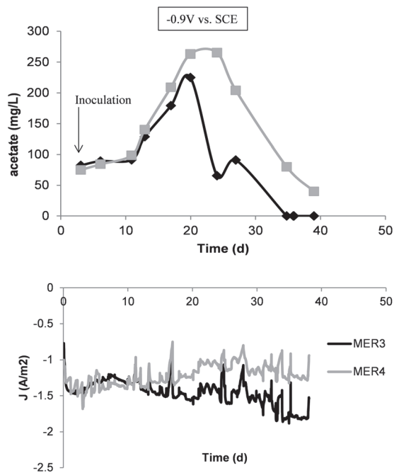
Fig. 3 Production of acetate and associated chronoamperometry in MERs polarized at -0.66 V vs. SHE for 40 days. On the 3rd day, the MERs were inoculated with the acclimated sludge.
