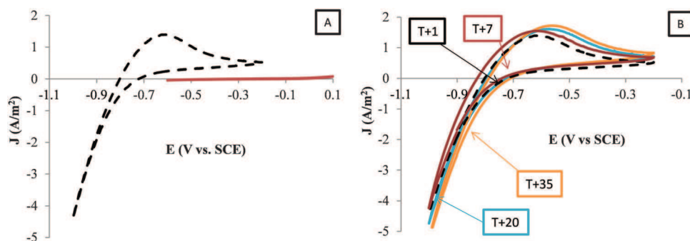
Fig. 4 Cyclic voltammeteries recorded at 1 \text{ mV s}^{-1} . (A) CV recorded before bacteria injection (abiotic) and after 1 day of polarization ( T + 1 ) at -0.36 V vs. SHE ( = -0.60 V vs. SCE) solid line and -0.66 V vs. SHE ( = -0.90 V vs. SCE) dotted line. (B) CV recorded at days 1, 7, 20 and 35 during the chronoamperometry at -0.66 V vs. SHE.
