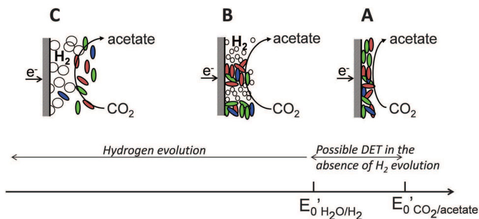
Fig. 10 Scheme of different potential zones relating to the conversion of \text{CO}_2 to acetate vs. hydrogen evolution. (A) Direct electron transfer can occur in the absence of hydrogen evolution; (B) direct electron transfer can occur in biofilm patches concomitantly to hydrogen evolution; and (C) strong hydrogen evolution precludes colonization of the electrode surface.
