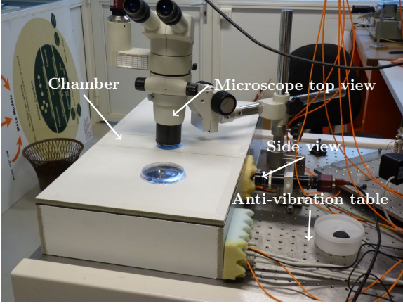
Figure 23: force sensor enclosed in a chamber on a antivibration table.
