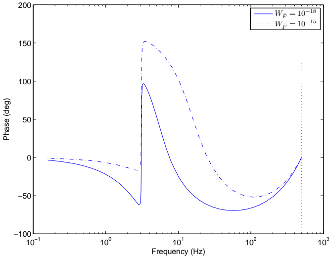
(b) Phase of H^K(\omega) ( f_s = 1000 Hz).
