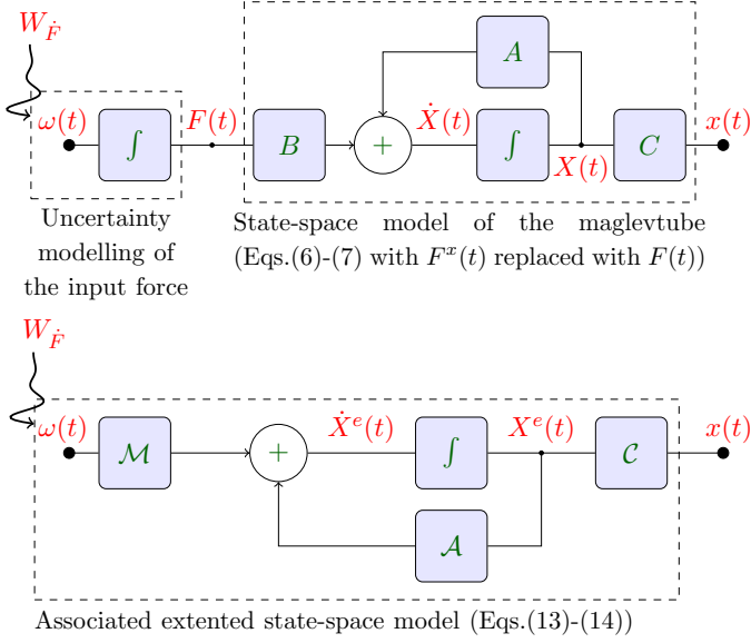
Figure 9: Blocks representation of the uncertain modelling of the input force and the deterministic model of the maglevtube.
