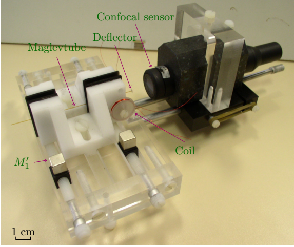
Figure 6: Force sensor prototype.
