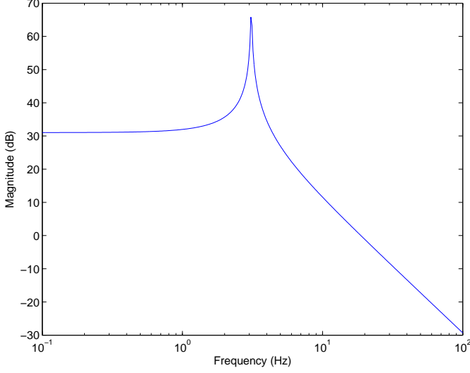
Figure 8: Simulated frequency response along x of the identified linear model.
