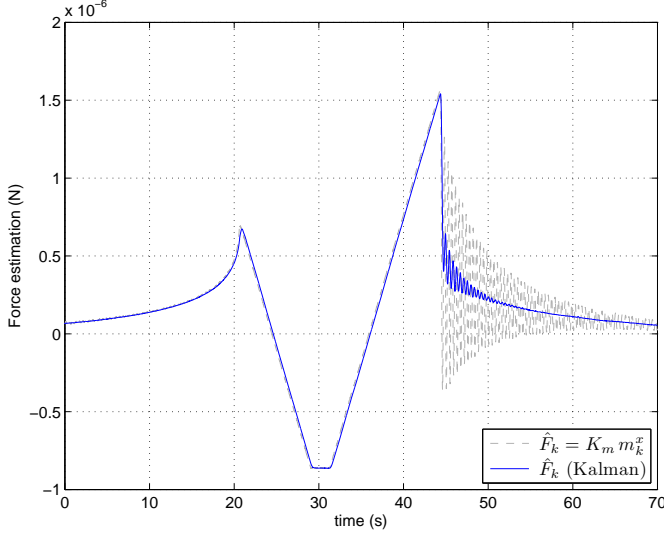
Figure 26: Experimental pull-off force measurement with non-contact attractive force also applied on the Maglevtube.
