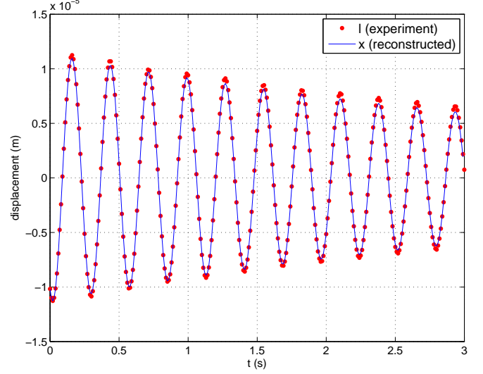
Figure 7: Measured and reconstructed zero input response (ZIR) of the maglevtube displacement.
