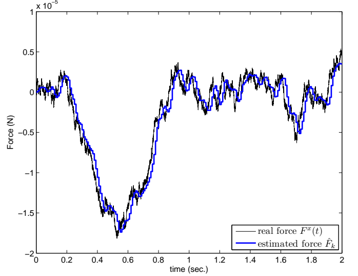
(a) Real and estimated force.
