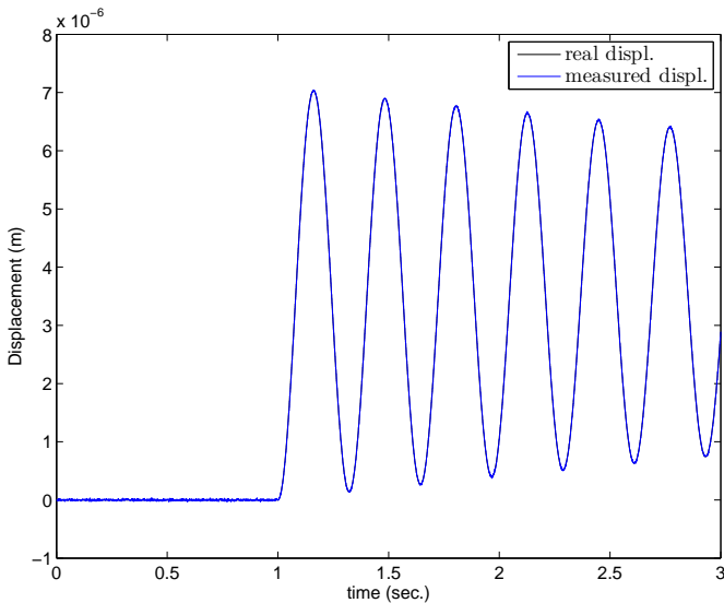
(c) Real and Measured displacement with f_s = 1000 \text{ Hz} .
