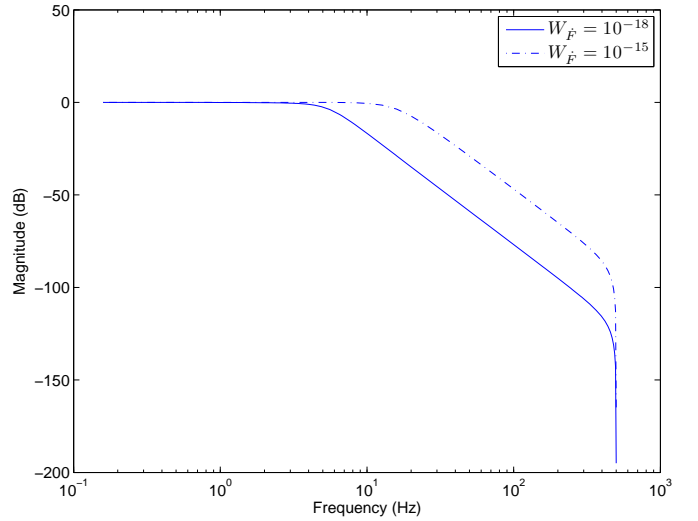
(b) Amplitude of H_g(e^{j\omega}) .
