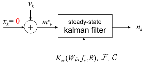
Figure 16: Output noise n_k in estimation \hat{F}_k due to the measurement noise v_k .
