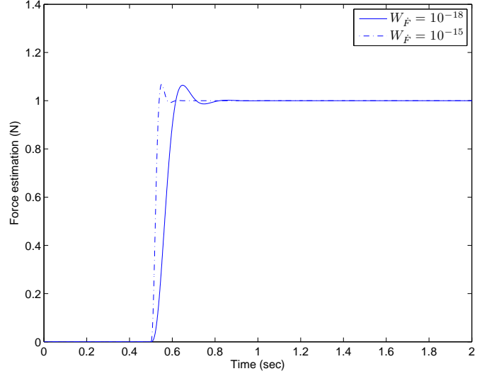
(a) Step force response with noise v_k set to zero.
