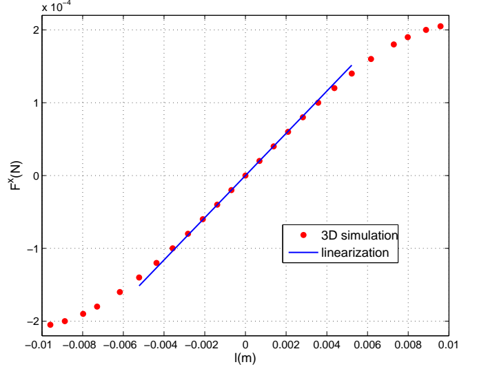
Figure 5: Simulated steady-state characteristic of the external force F^x versus the displacement x of the maglevtube.
