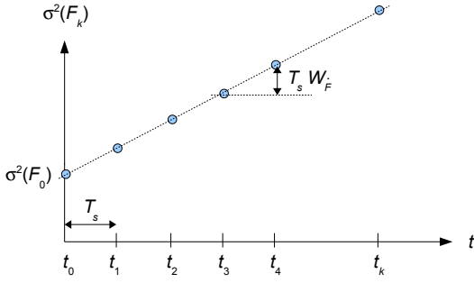
Figure 10: W_{\hat{F}} effect on the a priori variance \sigma^2(F_k) .
