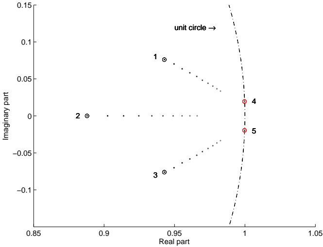
Figure 21: Impact of W_{\dot{F}} on the five eigen values (1 to 5) of A_g . The circled values are associated to W_{\dot{F}} = 10^{-15} \text{ N}^2/\text{Hz} .
