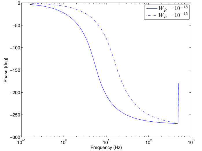
(c) Phase of H_g(e^{j\omega}) .
