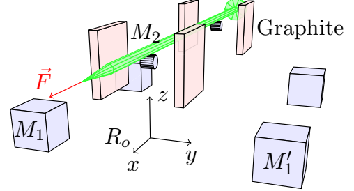
Figure 3: Levitating seismic mass in the force sensing device.
