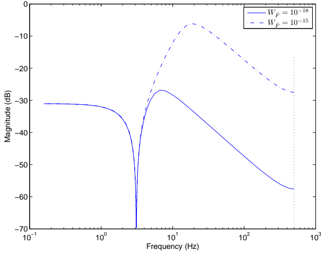
(a) Amplitude of H^K(\omega) ( f_s = 1000 Hz).
