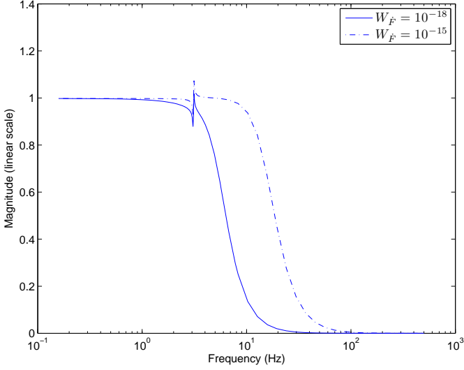
Figure 20: Global amplitude frequency response H_g(e^{j\omega}) with used calibration.
