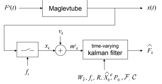
Figure 11: Force estimation with a time-varying Kalman filter.
