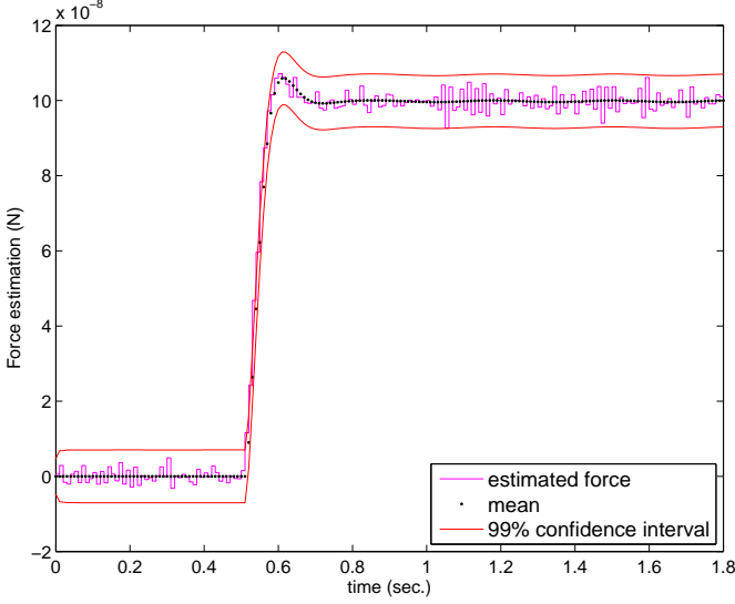
Figure 17: 99% confidence interval ( \pm 3\sqrt{\Sigma_k} ) on the force estimation with W_{\hat{F}} = 10^{-15} \text{ N}^2/\text{Hz} and f_s = 100 \text{ Hz} .
