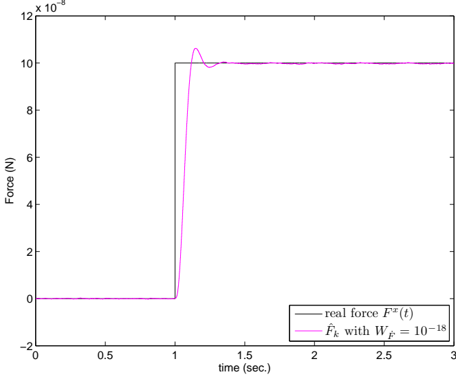
(a) Real and estimated force with W_{\dot{F}} = 10^{-18} \text{ N}^2/\text{Hz} .
