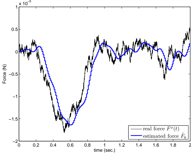
(a) Case W_{\dot{F}} < W ( W_{\dot{F}} = W/1000 ).
