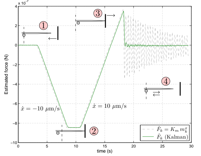
Figure 25: Experimental pull-off force measurement.
