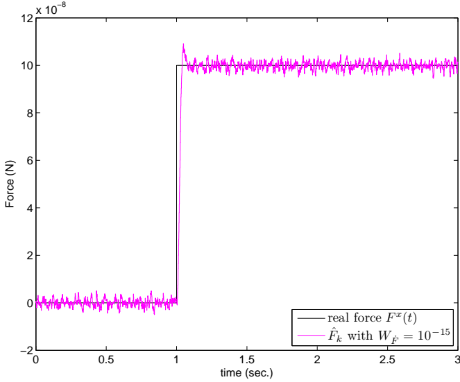
(b) Real and estimated force with W_{\dot{F}} = 10^{-15} \text{ N}^2/\text{Hz} .
