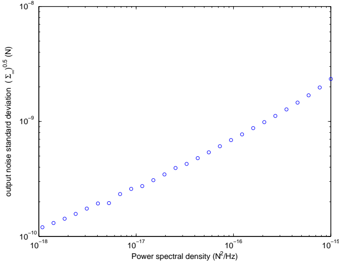
Figure 18: Standard deviation \sqrt{\Sigma_\infty} versus W_{\hat{F}} for f_s = 100 \text{ Hertz} and R = 1.44 \times 10^{-16} \text{ m}^2 . Small irregularities are mainly due to numerical errors during the solving of discrete Riccati equation to obtain K_\infty(W_{\hat{F}}, f_s, R) .
