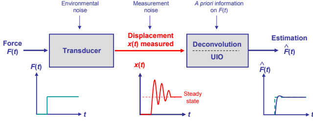
Figure 1: Force estimation using a deconvolution approach or an unknown input observer (UIO).
