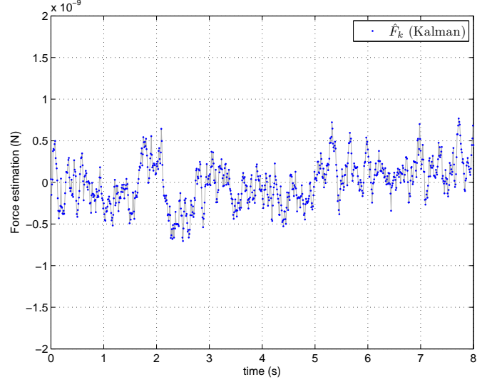
Figure 22: Measurement of the external disturbance force at 2:30 PM.
