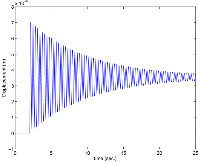
Figure 4: Simulated step response of the maglevtube with an external input force set to one micro newton.
