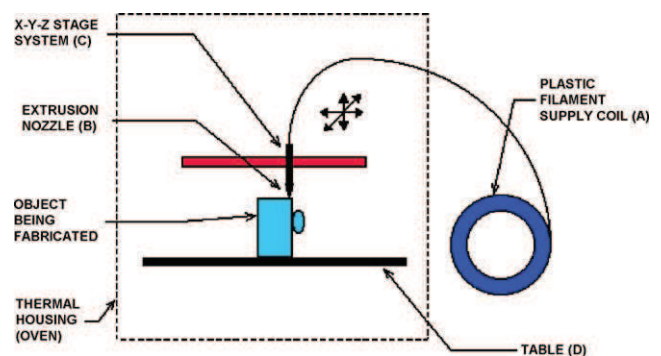
Fig. 6. Fused deposition modeling.
