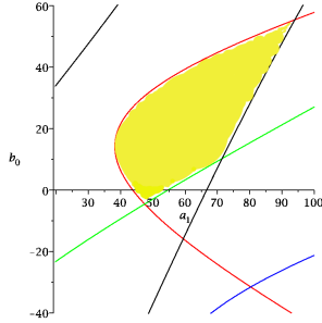
Figure 3: 4 conics
