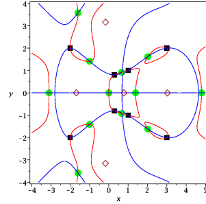
Figure 4: 20 roots
