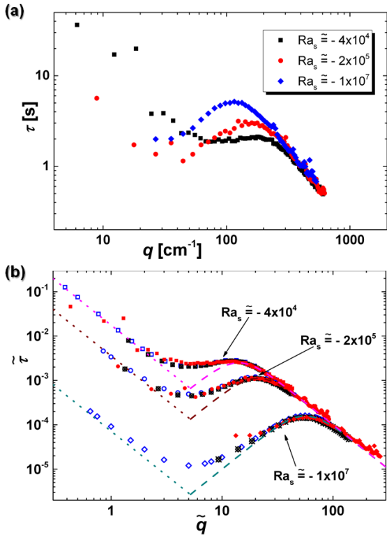
Fig. 3: Effective decay times: (a) Log-log plot of the experimental decay times \tau as a function of wave vector q for different Rayleigh numbers. (b) Same in terms of dimensionless variables. In panel (b), filled red symbols are experimental data, open blue are for calculations based on the FHD model, and open-crossed black are from numerical simulations. Dashed curves represent Eq. (2) for \tilde{q} > \tilde{q}_b , which accounts for gravity and diffusion only. Dotted lines represent Eq. (6) for \tilde{q} < \tilde{q}_b , which accounts for confinement.
