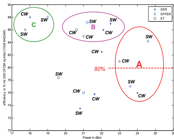
Fig. 10. PA efficiency versus PA output power, for EER, ET, EF-PER case, and for the same transistor in SW or CW mode (dynamical variation of V_{DS} and v_{rf} with the simulated OFDM signal).
