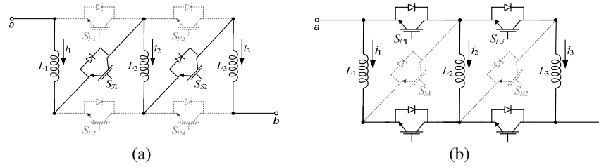
Fig. 3. The series-parallel inductor electronic circuit: (a) parallel mode operation; (b) series mode operation.
