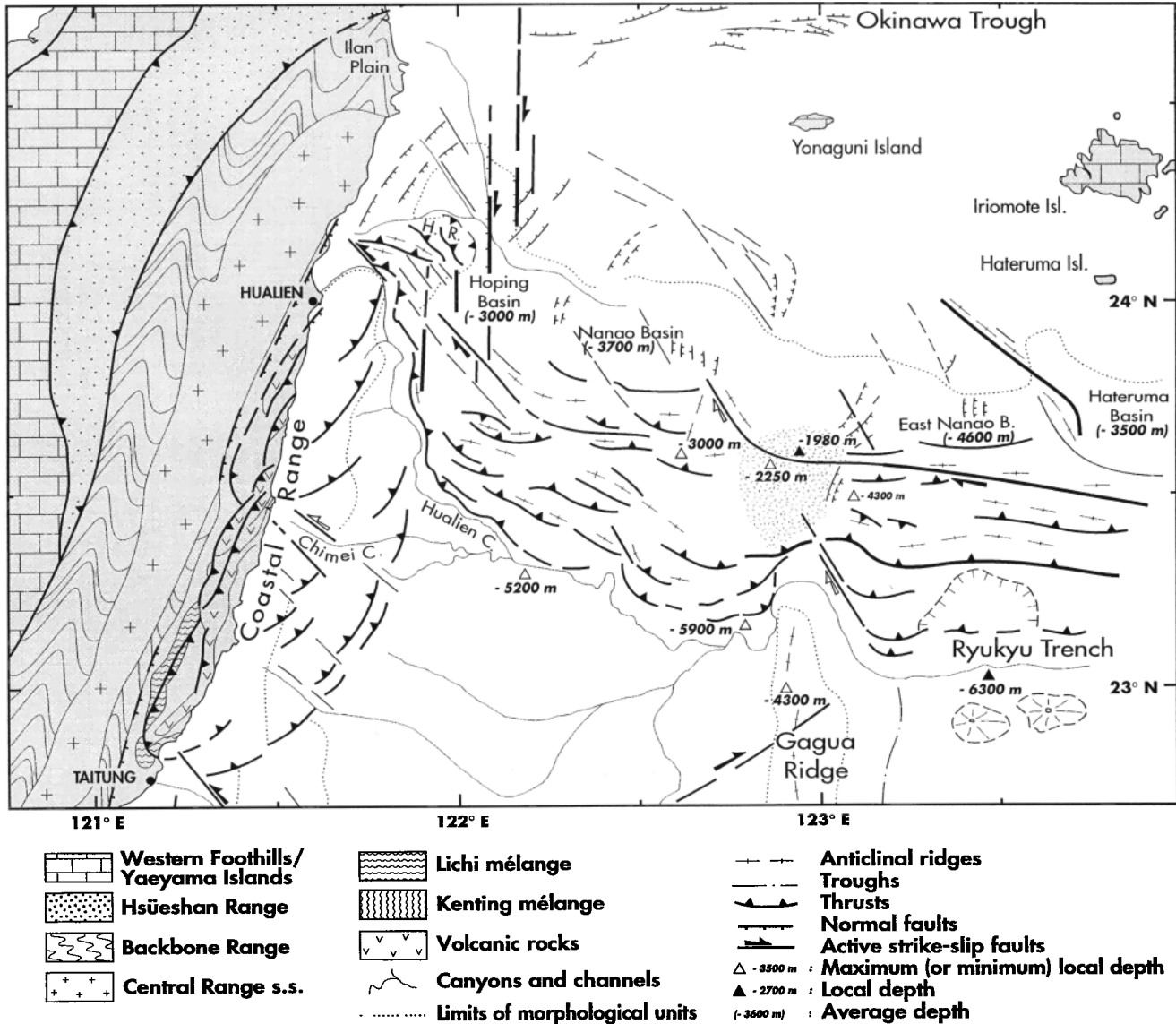
Figure 4. Simplified structural map of the study area offshore east of Taiwan, based on the analysis of all the ACT seismic lines, as well as 1/100,000 scale bathymetric charts. Simplified geology is given on land with more details along the Coastal Range. The stippled area represents the uplifted part of the accretionary wedge and forearc basin north of the Gagua Ridge. Normal faults in the Okinawa Trough are based on Sibuet et al. [1998]. HR is Hsincheng Ridge.
