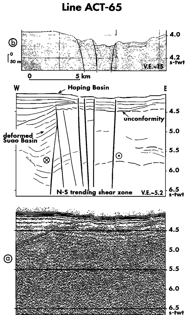
Figure 11. (a) E-W time-migrated 6-channel seismic line ACT 65 across the southern part of the Hopping Basin. The Hopping Basin sequences are thinning toward the east above the highly deformed Suao Basin strata [see Lallemand et al., 1997b]. The vertical strike-slip faults might belong to the N-S transform zone which allows the Ryukyu Arc to drift southward with respect to the SCB (see Figure 4). (b) A kind of flower structure is visible on the 3.5 kHz profile. The horizontal scale is the same as Figure 11a but vertical exaggerations differ. Vertical exaggeration is \sim 5 at seafloor on the seismic line and is \sim 15 on the 3.5 kHz profile. See location on Figure 3 and Plate 2.
