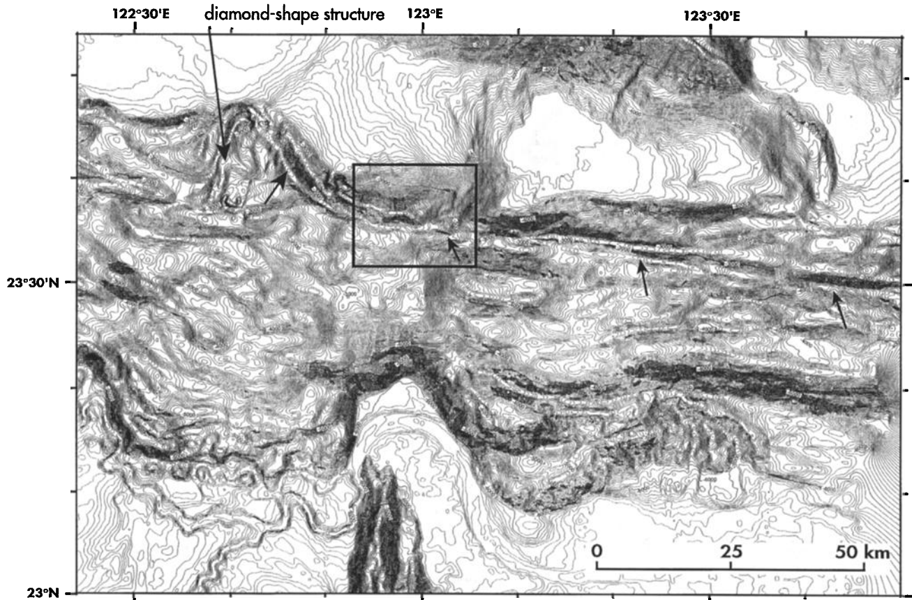
Figure 6. Bathymetric map of the Yaeyama accretionary wedge in the region of apparent interaction between the Gagaa Ridge and the margin (see location in Figure 3). Isobaths are every 20 m. Note the strike-slip fault at the rear of the wedge (small arrows) and the steepness of deformation fronts in and east of the reentrant along the emergence of the out-of-sequence thrust. A particular structure is observed at the rear of the wedge near 122°40'E, referred as the diamond-shaped structure in this paper (see explanations in the text). Location of Figure 7 (box).
