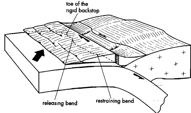
Figure 13. Perspective cartoon illustrating the geometry of releasing and restraining bends of the toe of the rigid backstop underlying the forearc basin sediments. The accretionary wedge is moving laterally along a major transcurrent fault located at the rear of the prism. This motion induces some dextral shearing within the forearc sedimentary section with stretching above the releasing bends and folding above the restraining bends of the arc basement.
