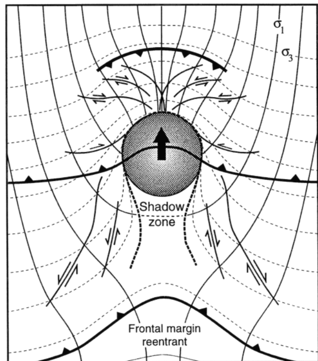
Figure 10. Shape of the stress field around the subducted seamount. The main thrusts and fault network, deduced from the experiments presented and previous morphological studies are superimposed.
