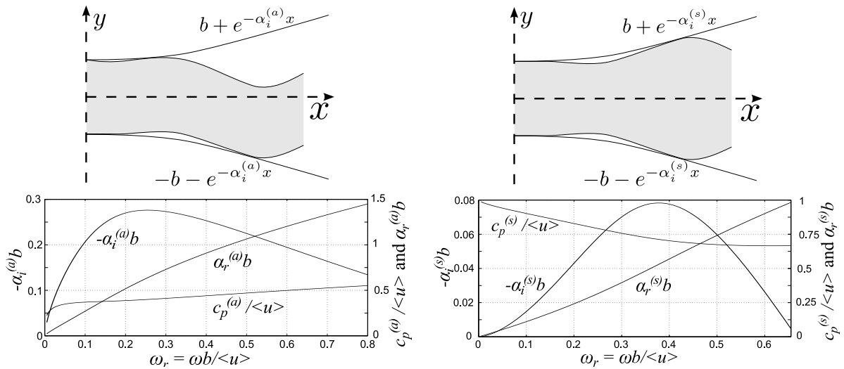
Figure 7: Top: Shape of the perturbation of the jet added to the mean flow for anti symmetric (left) and symmetric (right) cases. Bottom: Corresponding real phase velocity c_p = \omega/\alpha_r , real part \alpha_r and imaginary part -\alpha_i of the wave number \alpha as function of the Strouhal number \omega_r = \omega b/\langle u \rangle , obtained by numerical solution equation Eq. (5).
