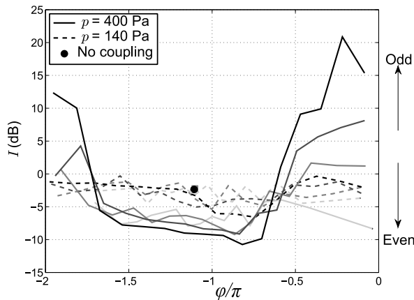
Figure 5: Un-parity index I (defined by Eq. (2)) as function of the phase of coupling \varphi for all gains (increasing gains with darker gray: G_p = -14 dB: black, G_p = -20 dB: lightest gray) and for two mean supply pressures (140 Pa et 400 Pa).
