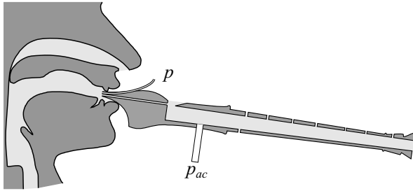
Figure 1: Sketch of the modified recorder that allows measurement of the acoustic pressure inside the bore and the pressure inside the mouth.
