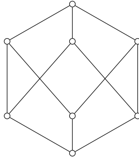
Figure 6: The context associated to a mode with three transpositions in the chroma system \mathbb{Z}_6 , its concept lattice and its simplicial complex. The latter consists of three tetrahedra, which should be embedded into some \mathbb{R}^N such that vertices with the same label are identified. If we consider the first three lines of the context only, then the concept lattice stays the same. As simplicial complex we get the boundary of a triangle, thus a space isomorphic to the circle S^1 . As shown in the text the latter is homotopy equivalent to the full simplicial complex depicted in the figure.
