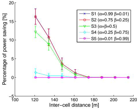
Figure 4: Power saving for the considered settings in WLAN scenarios.
