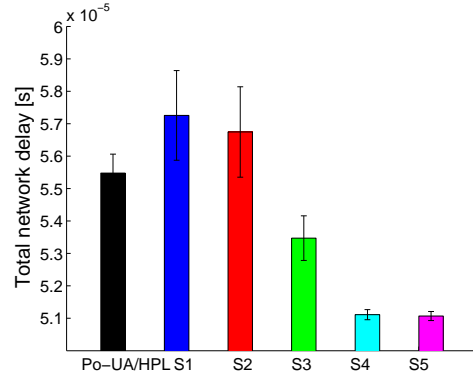
Figure 11: Total network delay for the considered settings and for Po-UA/HPL in LTE scenario for a urban deployment.
