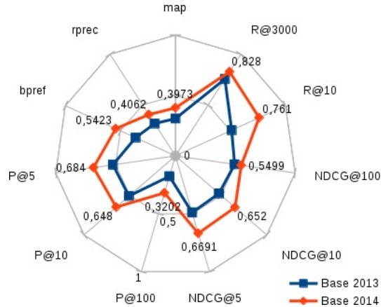
Figure 1. Performance of the baseline setting, without application of the query expansion.
