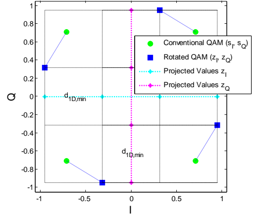
Fig.1. Conventional QPSK (s_i, s_\varrho) , rotated QPSK (z_i, z_\varrho) , projected values of rotated QPSK signal and d_{1D, \min} = 2\beta_s \sin \theta .
