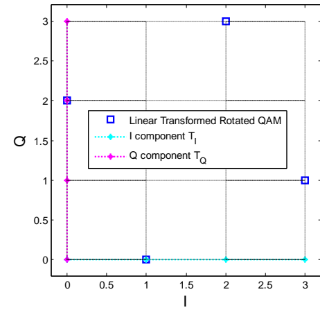
Fig.2. Linear transformed rotated QPSK (T_i, T_\varrho) from (z_i, z_\varrho) by using (12) and (13).
