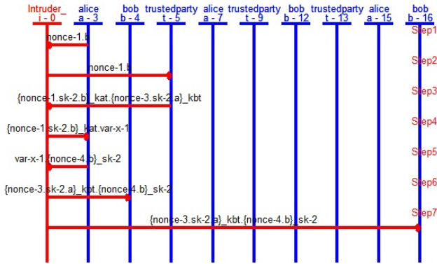
Fig. 6: An MSC of the replay attack detected by AVISPA against ISO/IEC 9798-2 unilateral authentication involving TTP. The attack is detected by OFMC backend and the MSC is generated by using the SPAN tool.
