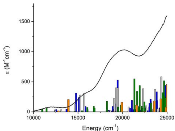
Figure 13. UV–vis spectrum of [Ru 2 (chp) 4 ] generated in CH 2 Cl 2 , compared to the TD-DFT-predicted electronic transitions for Ru 2 (chp) 4 (orange), Ru 2 (chp) 4 (CH 2 Cl 2 ) (green), 7 (blue), and 8 (gray).
