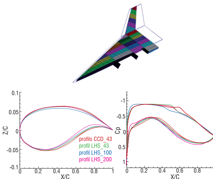
Figure 11 – Structure and aerodynamics, RSM test cases
