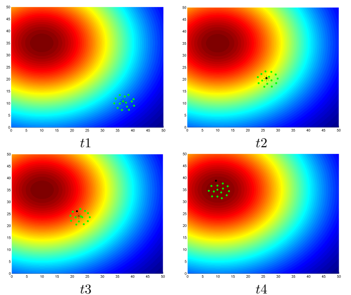
Figure 2. Maximum seeking of a field with fleet reconfiguration
