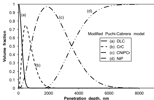
Fig. 8. Change in the volume fraction of each coating contributing to the composite hardness, according to the PC model, as a function of penetration depth.
