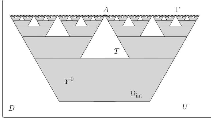
Figure 3: An exemple of the domains \Omega_{\text{int}} and \Omega_{\text{ext}} in the case \theta = 0
