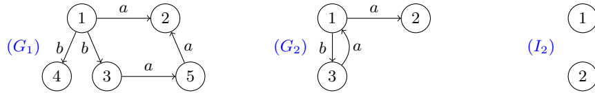
Fig. 1. Ambiguous graph G_1 and unambiguous graph G_2 .
