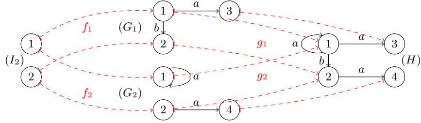
Fig. 4. A “synchronization” pushout example.
