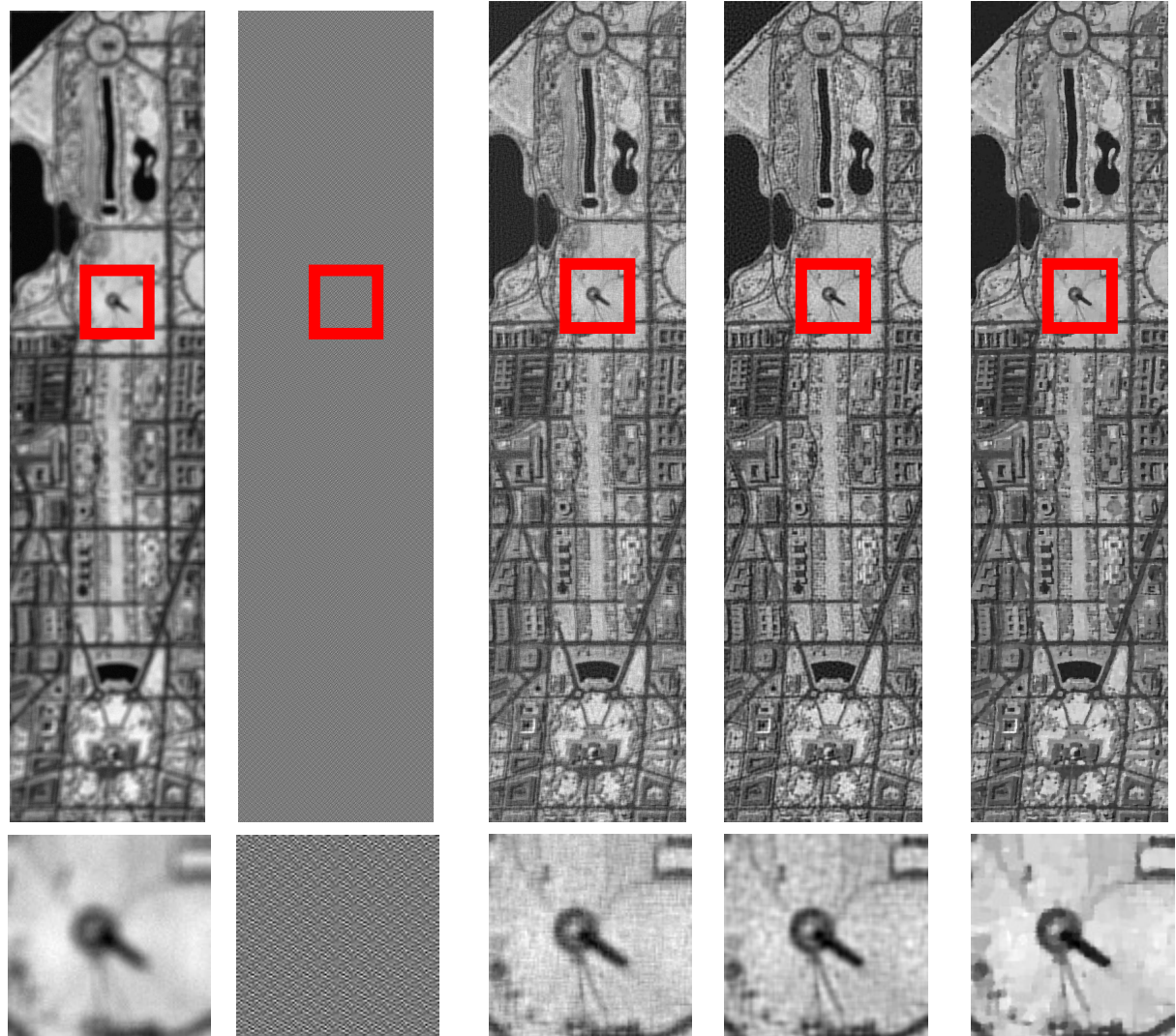
(a) Degraded Uniform blur 9 \times 9 Gaussian noise (b) Inverse filtering (c) Quadratic regularisation \Lambda = \text{Id} (d) \Lambda Laplacian (e) Total variation
