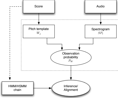
Figure 1: Architecture of the Antescofo system.
